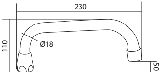
BICA "U" UNIVERSAL CAÑO "U" UNIVERSAL | UNIVERSAL "U" SPOUT | BEC "U" UNIVERSEL
